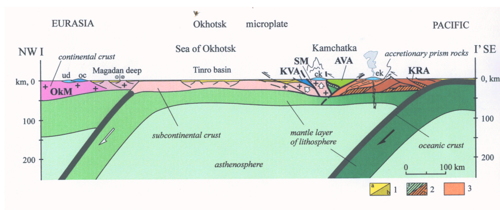
Figure 2. Simplified cross-section locating in Fig. 1 of Northeast Sea of Okhotsk and Kamchatka. Data on type and thickness of crust are taken from Kharakhinov et al. (1996). Subduction zones of the Okhotsk microplate and the Pacific plate are shown after Gorbatov et al. (2000). Black and white arrows indicate active and inactive subduction, respectively. In letters: Uda-Murgal volcanic-plutonic belt (ud); Okhotsk microcontinent (OkM). Other key symbols as in Fig. 1. 1 = Cenozoic (a) and Cretaceous (b) sedimentary units; 2 = oceanic basement of AVA (a) and KRA (b); 3 = oceanic crustal unit of Vetlovka intraarc basin.
