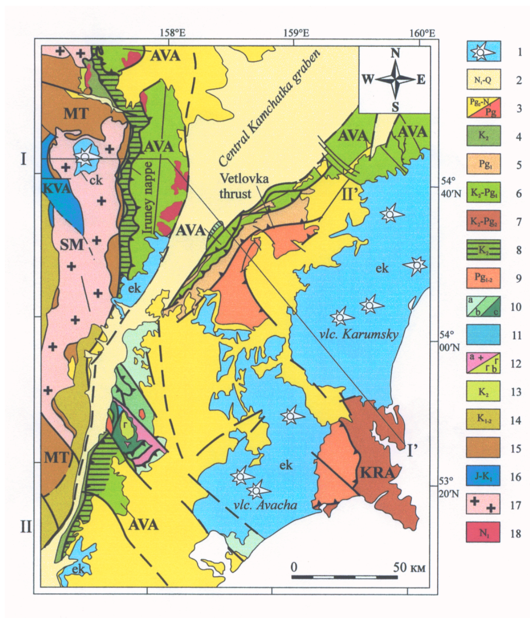
Figure 3a. Tectonic map of Southern Kamchatka. Cross-section along line I-I' is shown in Fig. 3b. 1-3 = overlap volcanic (1) and sedimentary (2-3) units; 4-9 = allochthonous units: 4-5 = continent-derived turbidites; 6 = Achaivayam-Valaginskaya (AVA) arc; 7 = Kronotskaya (KRA) arc; 8-9 = oceanic crustal units of Irunev (IB) marginal basin (8) and Vetlovka (VB) intraarc basin (9); 10-12 = Ganalsky syncollisional metamorphic core; 13-17 = Sredinny microcontinent: 13-14 = molasse (13) and turbidites (14); 15-16 = metamorphosed arc terranes Malkin (MT) (15) and Kvachona (16); 17 = granulite basement; 18 = granites. Horizontal hatched pattern on the map is vertical on the cross section. Other symbols as in Figs. 1, 2.
