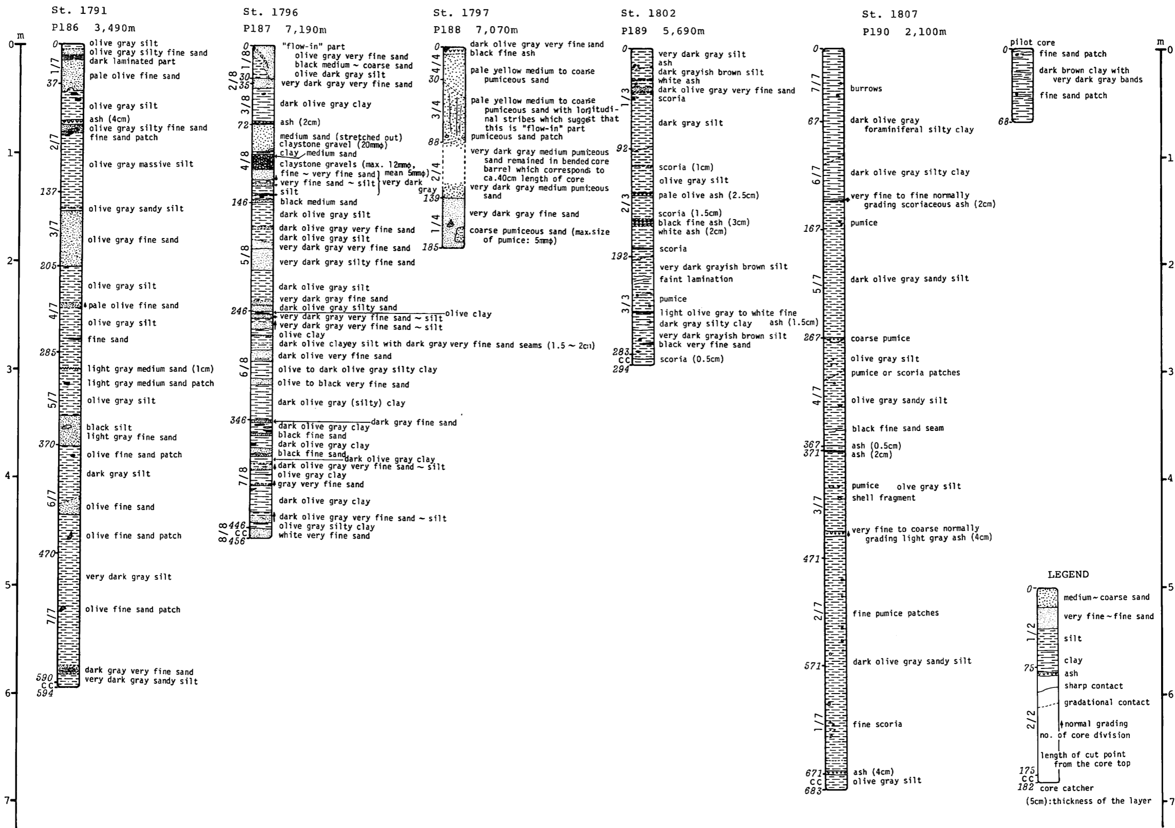
Fig. XV-5 Columnar sections of the cores taken from the northern area of the Ogasawara Arc.
