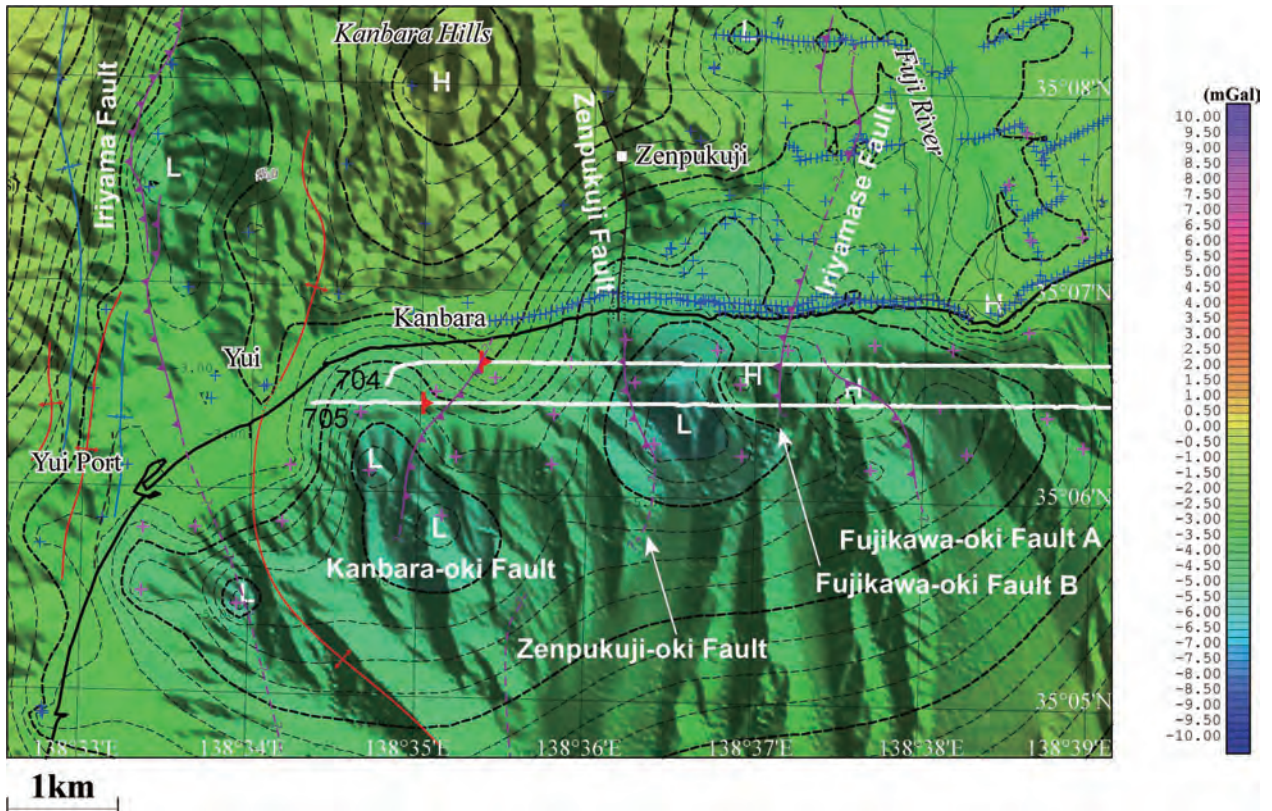
第 5 図 詳細検討範囲（蒲原地域）の残差重力図。仮定密度は 2.3\text{g/cm}^3 。コンター間隔は 0.25\text{ mGal} 。実線及び破線のコンターは各々正值と負値を示す。H と L は、各々高重力異常と低重力異常を示す。青の十字：既存の重力測点。ピンクの十字：海底重力測点及び新規の陸上測点。白の実線と赤の断層記号は各々反射法音波探査（佐藤・荒井，2016）による測線位置と反射断面で東傾斜の逆断層が認められた地点を示す。背景の陰影図は地形。黒、紫、赤及び青の線は、各々、断層、活断層、背斜及び向斜（尾崎ほか，2016b）を示す。 Fig.5 Residual Bouguer anomalies in the detailed study area (Kambara area) with the removal of 1\text{km} upward-continuation (Fig. 3) from the Bouguer anomalies (Fig. 2). Assumed density is 2.3\text{g/cm}^3 . Contour interval is 0.25\text{ mGal} . Solid and broken lines indicate positive and negative values, respectively. H and L signs show gravity highs and lows, respectively. Blue crosses: Pre-existing gravity stations. Pink crosses: Ocean bottom gravity stations and newly observed land gravity stations. White solid lines denote seismic reflection survey lines (Sato and Arai, 2016). Red fault symbols show the locations where east-dipping reverse faults were found by the seismic reflection survey (Sato and Arai, 2016). Shaded terrain relief is superimposed. Black, purple, red and blue lines denote faults, active faults, anticlines and synclines after Ozaki et al. (2016b), respectively.
