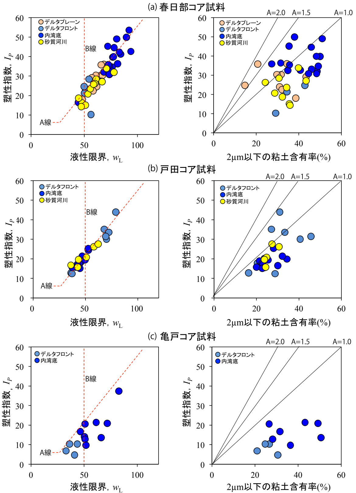
第6図 各コア試料の塑性図と活性度. Fig.6 Plasticity chart and activity.
